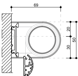
32.210.xx.xx Montageprofiel Wandmontage
